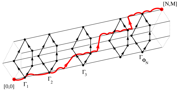
FIG. 2. The skeleton for the slab graph and a longest path.
