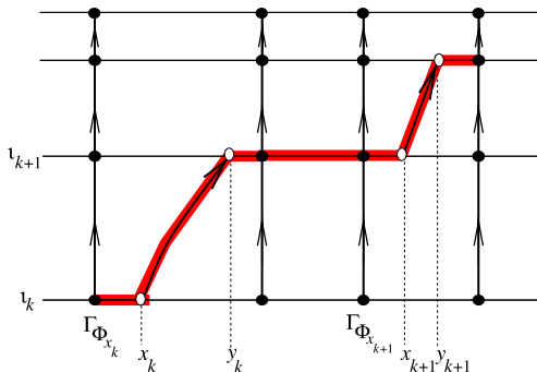
FIG. 3. Construction used in obtaining the upper bound.
